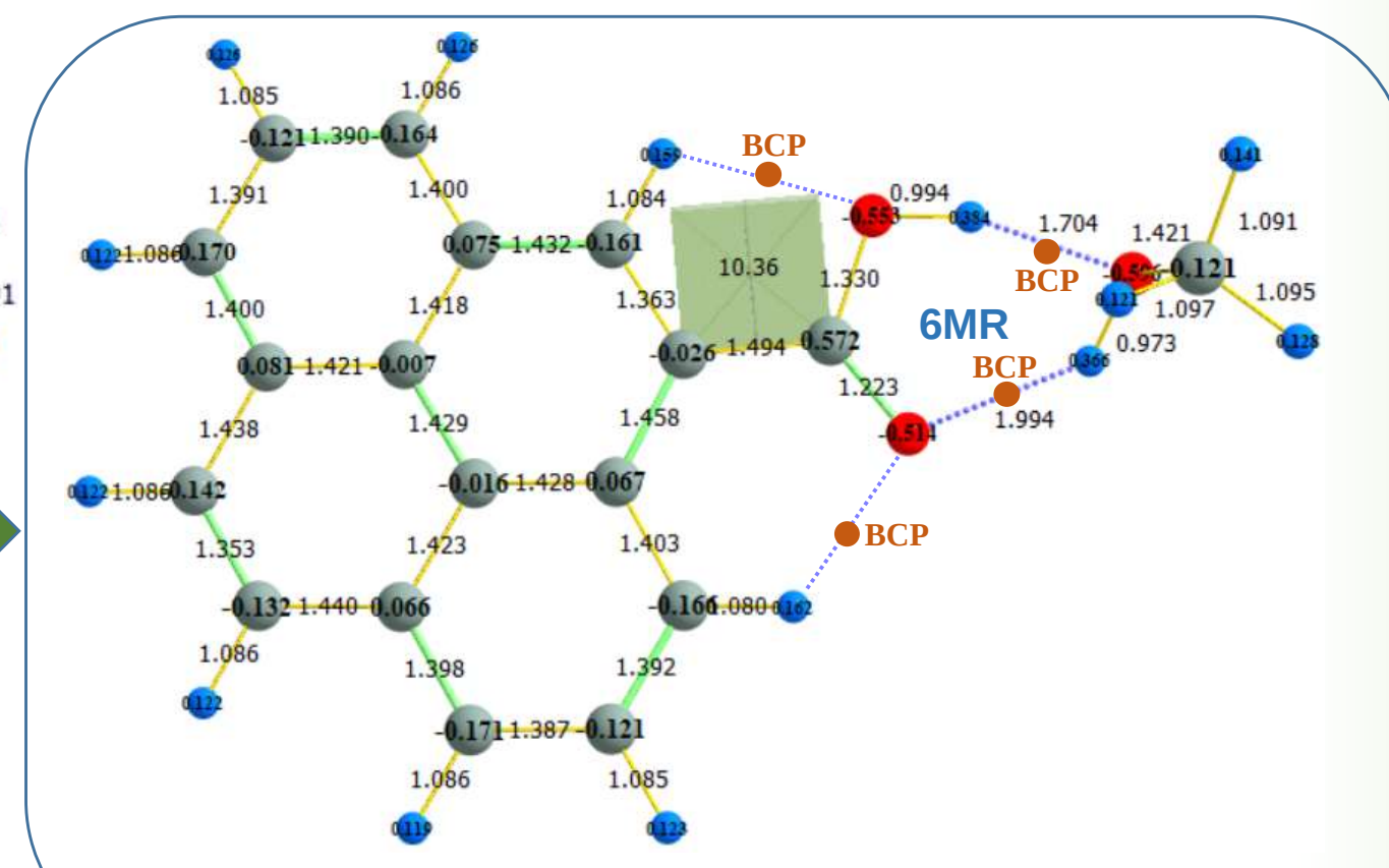
Cyclic Complex b (CCb)
