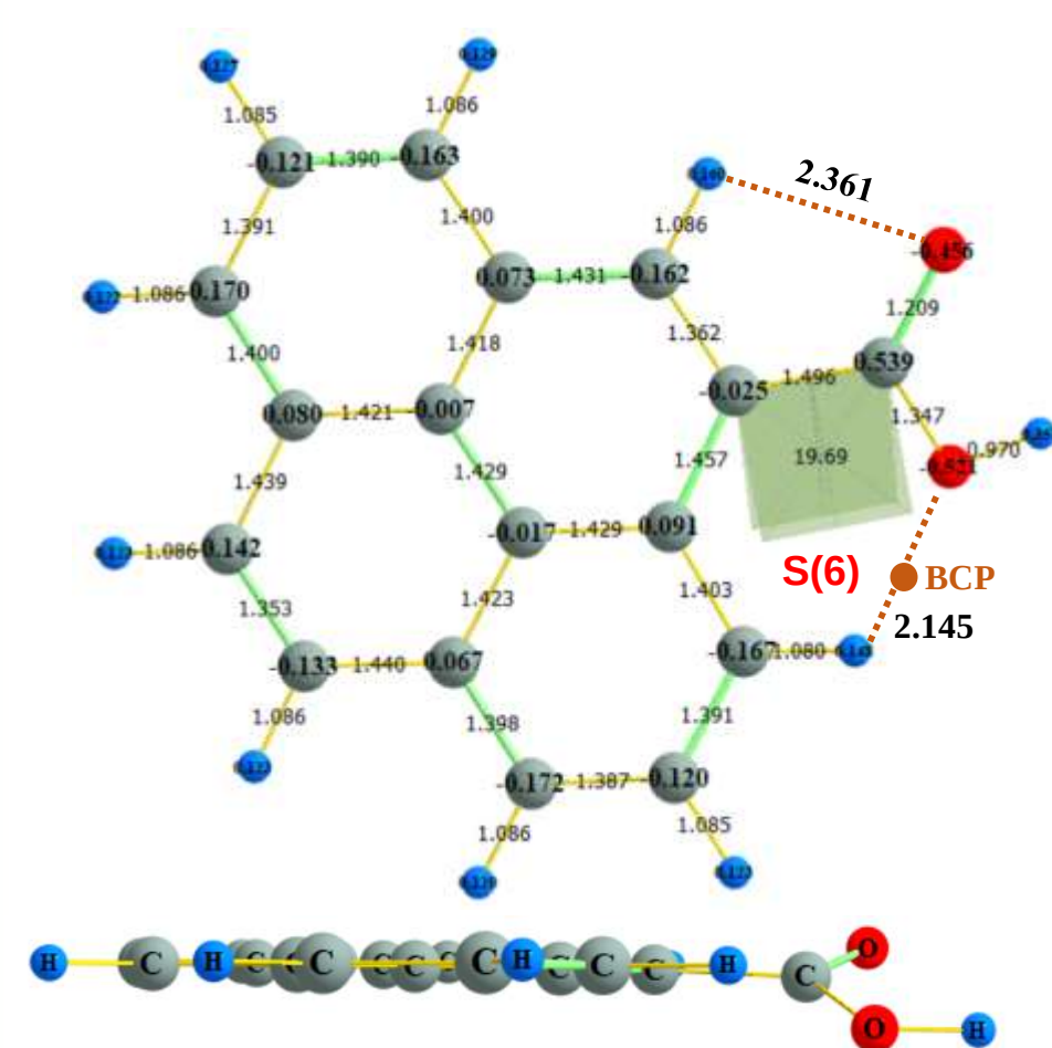
Pyr-COOH (A) E_{\text{total}} -804.02749406 Eh
