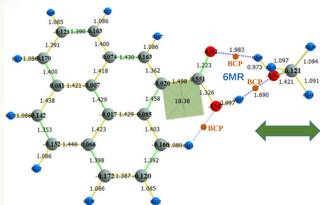
Cyclic Complex a (CCa)
