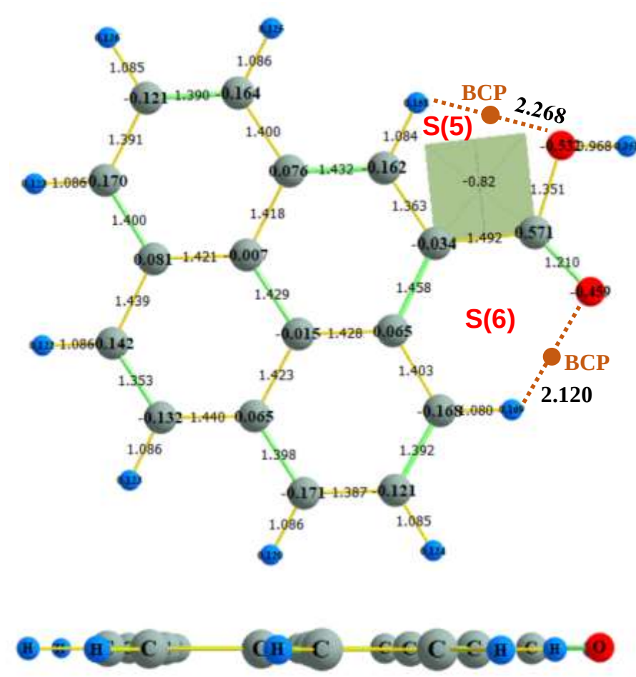
Pyr-COOH (B) E_{\text{total}} -804.02976006 Eh
