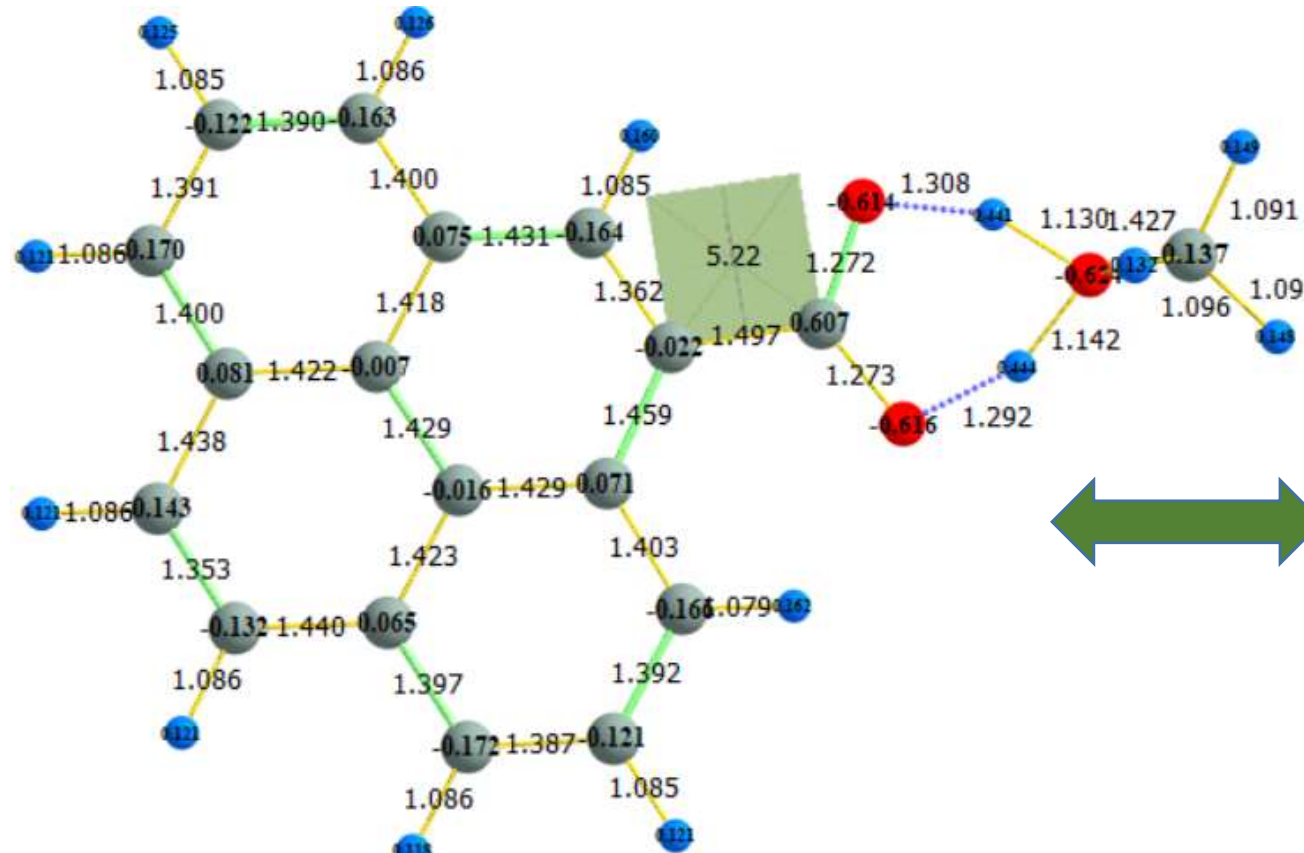
Transition state (TS)
