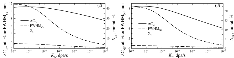
Figure 1: Production rate dependence of surface Cr depletion \Delta C_{Cr} and Ni enrichment \Delta C_{Ni} (solid line), FWHM_{Cr} and FWHM_{Ni} (dashed line) and segregation area of Cr S_{Cr} and Ni S_{Ni} (dash-dotted line). Calculations were performed at temperature T = 400 \sim 600^\circ C , dose D = 10 -dpa (displacement per atom).
